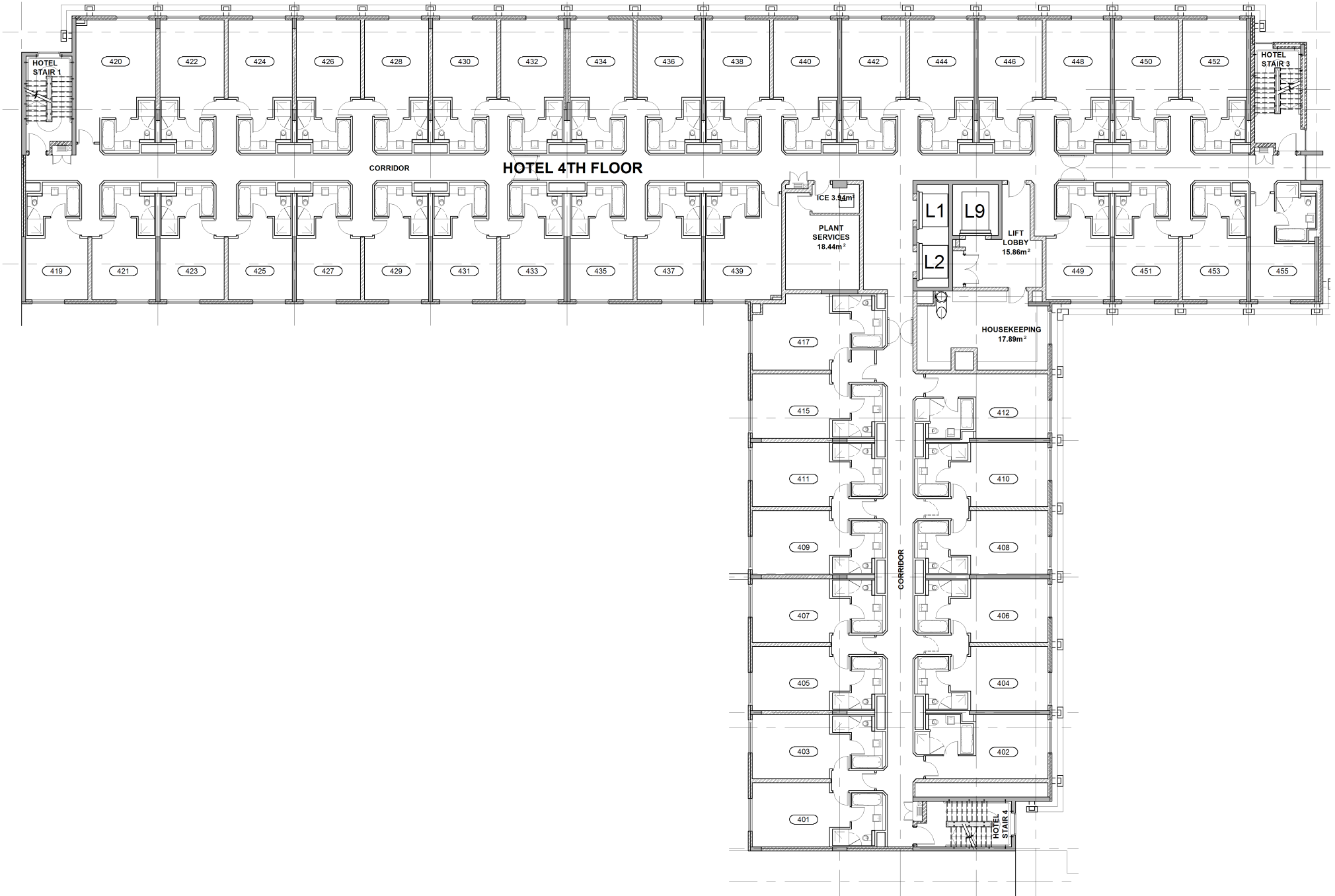
HOTEL FOURTH FLOOR
