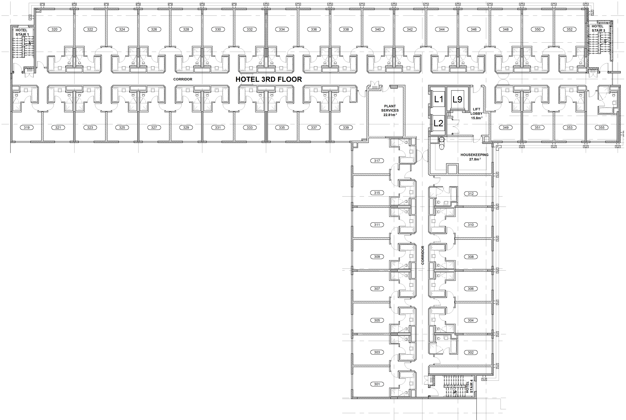
HOTEL THIRD FLOOR
