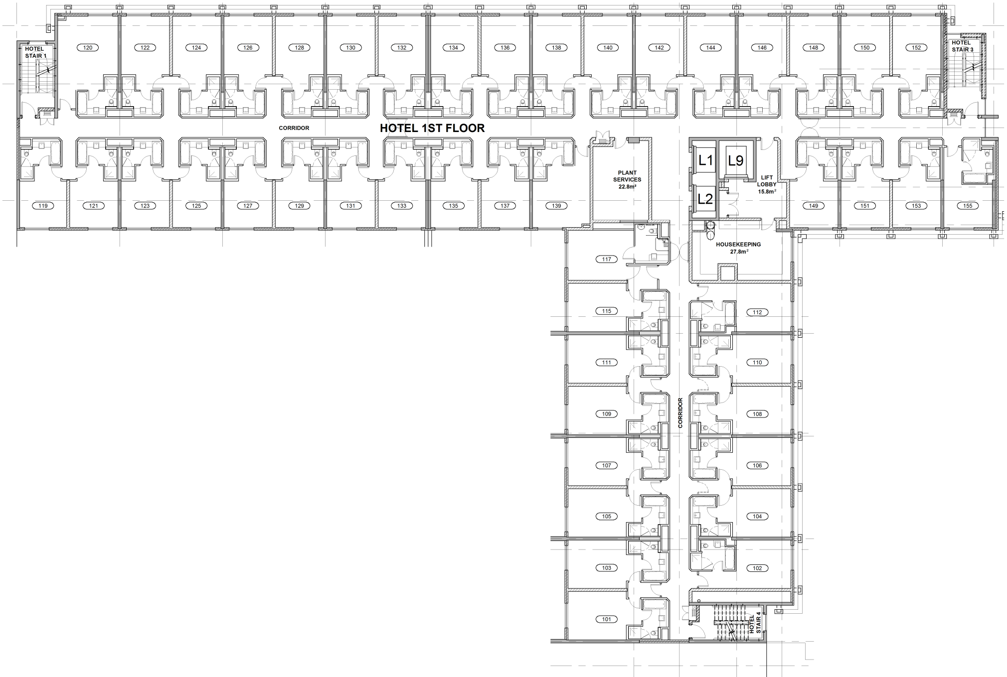
HOTEL FIRST FLOOR
